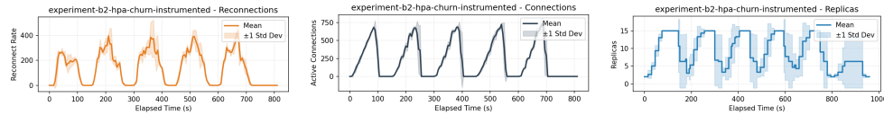
Fig. 4 Multi-run averages from Experiment B2-Instrumented demonstrating that HPA scale-down events directly trigger severe reconnection storms and connection instability. Left: Reconnection rate showing peak observed average rates of 512 connections/second perfectly synchronized with scale-down events. Center: Active connection count showing instability induced by simultaneous bursts, peaking at a mean of 767 ( \pm 46 ). Right: HPA replica changes, confirming that each downward step causes the corresponding session disruptions.
