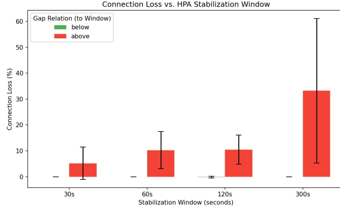
Fig. 6 Connection loss percentage relative to the HPA stabilization window and gap duration. Green bars (“below”) show zero loss when the gap is shorter than the window; red bars (“above”) show consistent connection destruction when the gap exceeds the window, regardless of window size.
