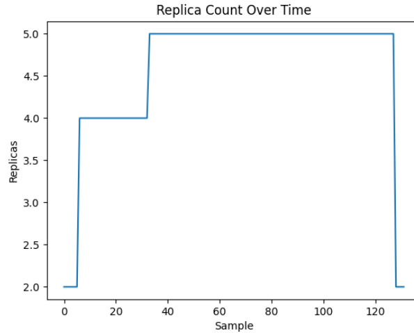
Fig. 2 Results from Experiment A establishing a correct-behavior baseline. Under monotonic Web-Socket load where CPU is artificially coupled to session count via continuous pinging, the clean staircase ascent, flat stabilization plateau, and controlled descent to the minimum demonstrate that HPA achieves the theoretical ideal only when signal-to-demand correlation is perfect.
