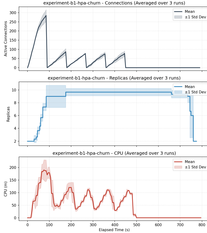
Fig. 3 Representative result from Experiment B1 demonstrating severe HPA over-provisioning and delayed recovery under cyclic load. HPA saturates at 10 replicas, a 233% over-provision relative to the connection-derived optimum of 3 replicas, and requires ~650 seconds to recover. Shaded bands show \pm 1 SD across 3 replications.
