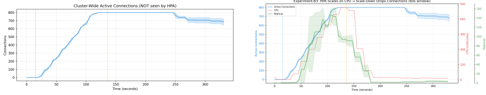
Fig. 5 Representative result from Experiment B3 showing staircase session destruction following successive HPA scale-down events. Left: Active connection count exhibits permanent staircase destruction ( 800 \rightarrow 771 \rightarrow 708 \rightarrow 644 ). Connections are irrecoverable under reconnect: false . Right: Combined signal view demonstrating that as CPU utilization (red) drops to near zero due to idle connections, HPA scales down (green), causing the permanent destruction of active sessions (blue).
