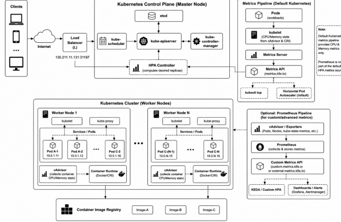
Fig. 1 Overview of the standard Kubernetes Horizontal Pod Autoscaler (HPA) control architecture. The diagram was created by the authors based on the Kubernetes HPA architecture described by Nguyen et al. [4] and the official Kubernetes architecture.
